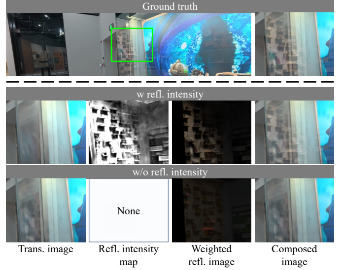
Fig. 9. Without the reflection intensity, the reflection color input to our model no longer adheres to the required linear color space, which hampers accurate reflection modeling and leads to degraded rendering quality.
