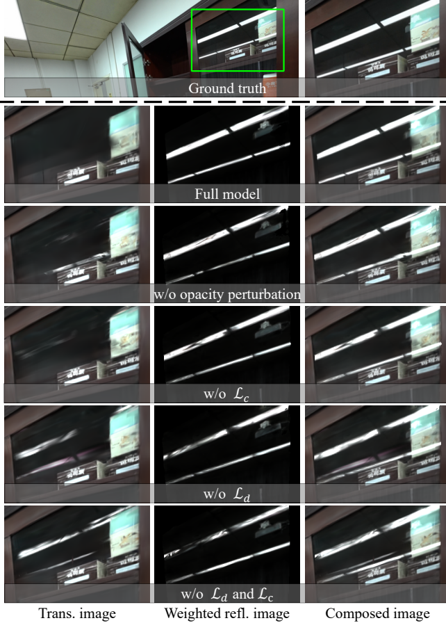
Fig. 8. Ablation results of regulations and opacity perturbation in Bookcase2 . The removal of either component leads to degraded decomposition, highlighting the importance of their joint contribution to realistic rendering.
