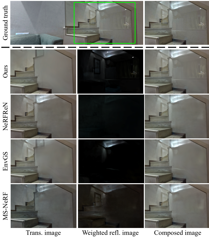
Fig. 6. Decomposition results in Loft compared with NeRFReN [3], MS-NeRF [30], and EnvGS [35]. Our method achieves comparable decomposition results and better novel view synthesis quality.
