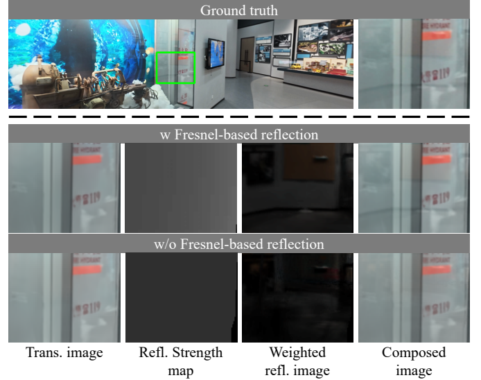
Fig. 10. Ablation results of Fresnel-based reflection in Ship . Without it, the model fails to capture view-dependent reflection strength, especially at grazing angles, which results in blurrier outputs.
