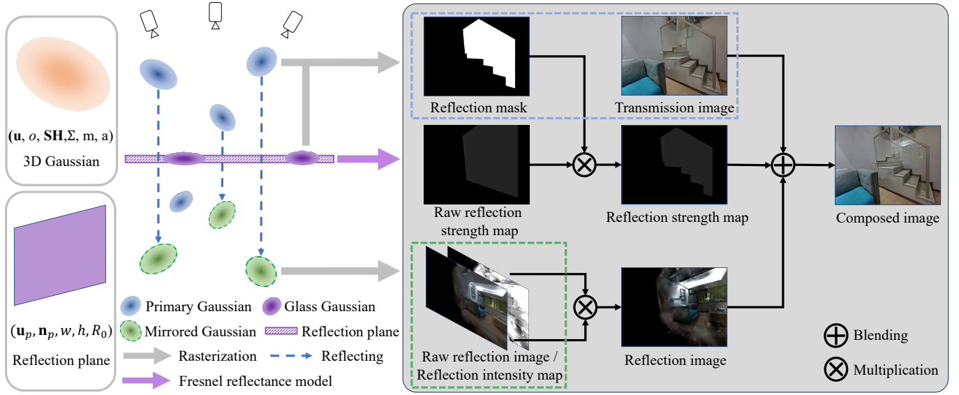
Fig. 1. Our rendering pipeline. The pipeline consists of two rendering passes. In the first pass, we render the transmission image C_t using primary Gaussians, and generate the reflection mask M by rendering both primary and glass Gaussians. We then compute the raw reflection strength map R_{raw} using Fresnel reflectance model, and multiply it with the reflection mask M to obtain the reflection strength map R . In the second pass, we mirror the primary Gaussians across the reflection plane P to produce the mirrored Gaussians, which are rasterized to generate the raw reflection image C_r and the reflection intensity map A . These two are multiplied to produce the reflection image C_r . Finally, we blend the transmission image C_t and the reflection image C_r using the reflection strength map R to produce the final image.
