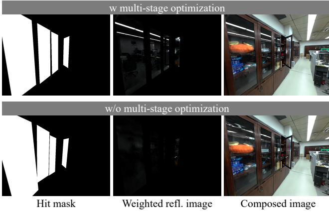
Fig. 11. Disabling multi-stage optimization leads to reflection plane drift and poor separation of reflection and transmission, demonstrating that it is crucial for accurate reflection modeling and high-quality rendering.
