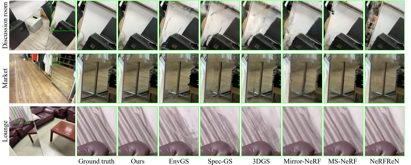
Fig. 4. Qualitative comparison on Mirror-NeRF dataset. Regions with noticeable differences are cropped and shown side-by-side for clear comparison.
