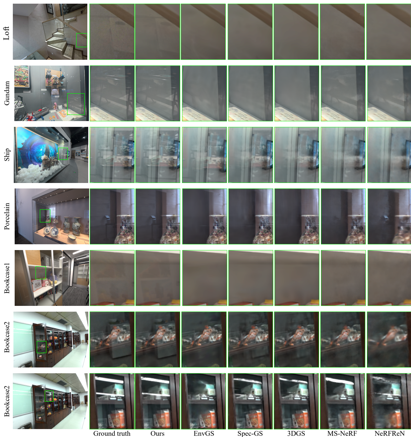
Fig. 3. Qualitative comparison with EnvGS [35], Spec-Gaussian [34], 3DGS [1], MS-NeRF [30] and NeRFReN [3] on the RTR dataset. We show images rendered from novel test viewpoints. Compared to these baselines, our method produces more accurate and detailed reflections, and yields results closest to the ground truth.
